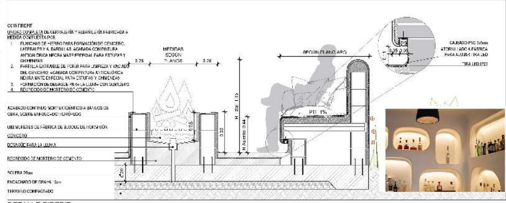
DETALLE FIREPIT
